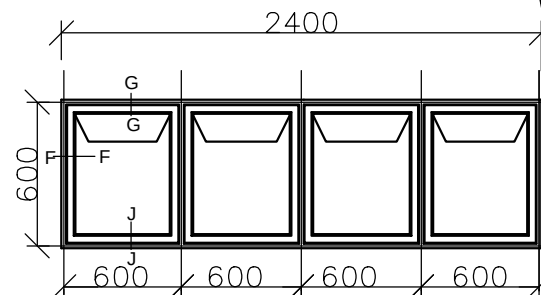
WINDOW TYPE W1V1
