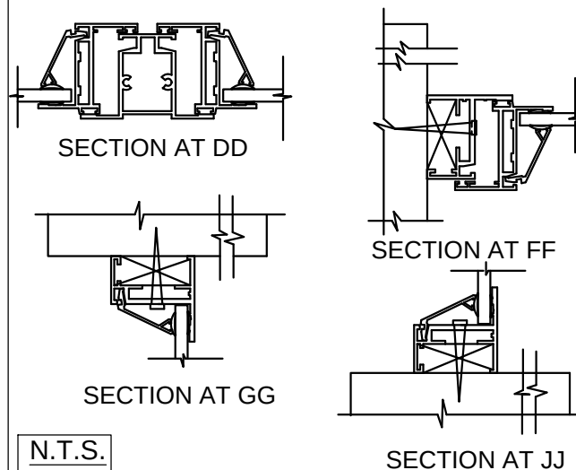
TYPICAL WINDOW AND VENTILATOR GRILL DETAIL
