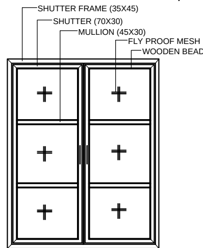
TYPICAL WINDOW AND VENTILATOR FLY PROOF DETAIL
