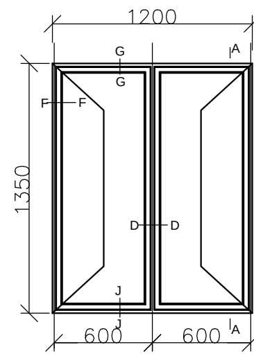
WINDOW TYPE W2V2
