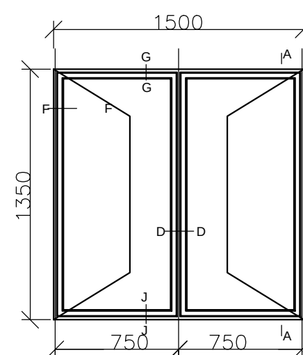
WINDOW TYPE W1V1
