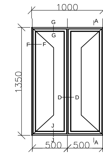
WINDOW TYPE W3V3
