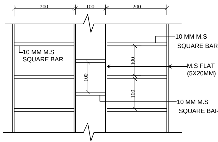
TYPICAL WINDOW AND VENTILATOR GRILL DETAIL
