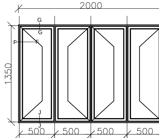
WINDOW TYPE W/V
